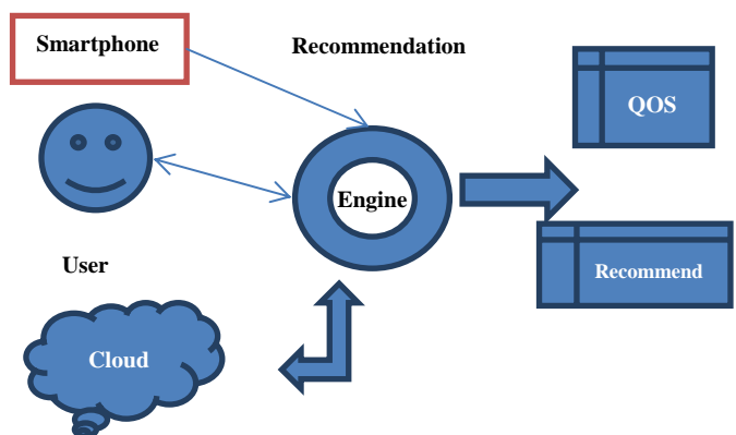
Figure 1: System Model
